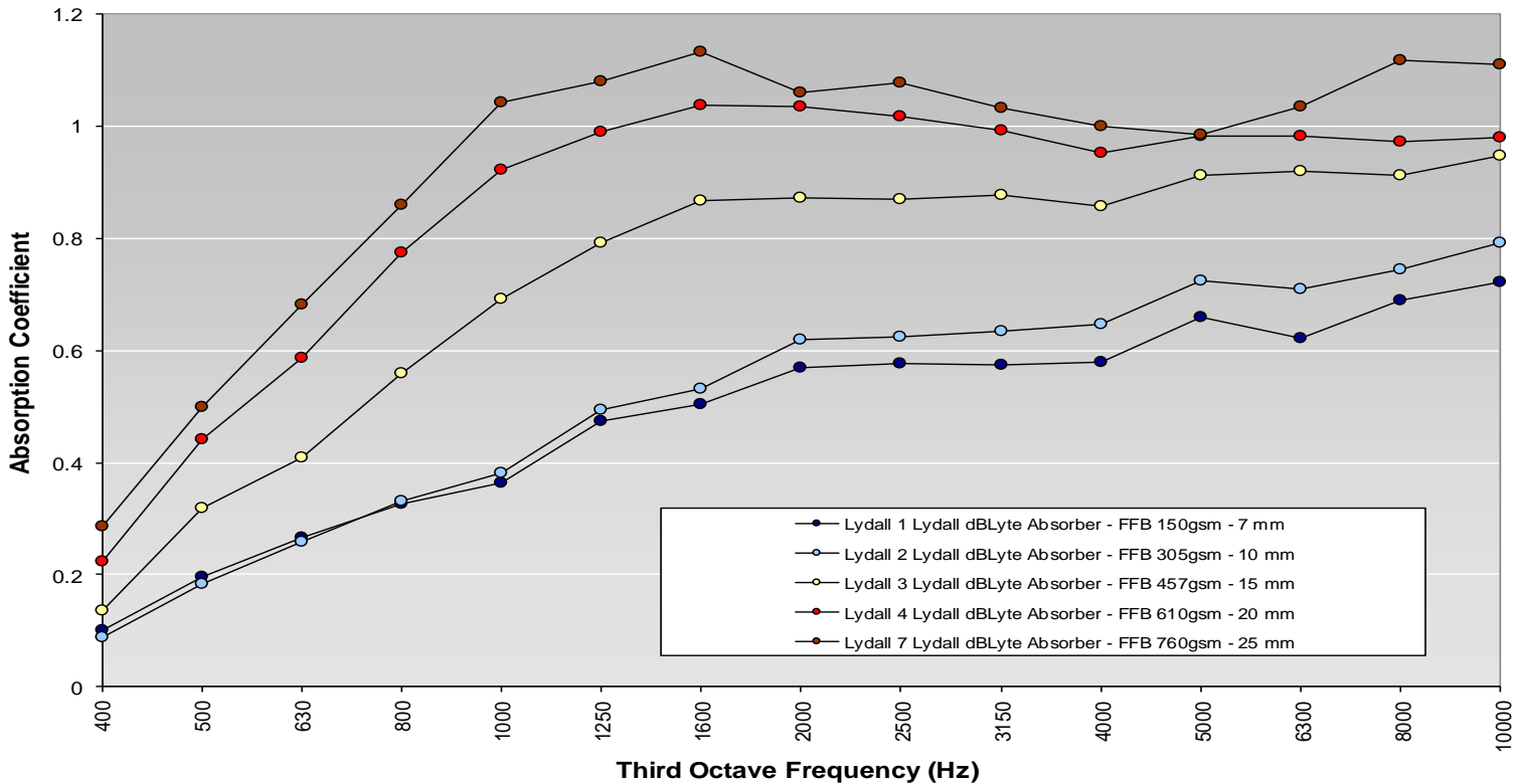
Lydall Random Incidence Sound Absorption
